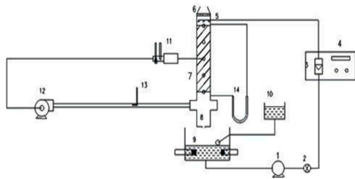
Figure (2) Experimental rig of forced draft counter flow water cooling tower.
