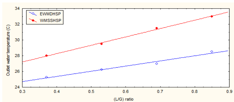
Figure (8): Variation outlet water temperature with (L/G) ratio for two packs.
