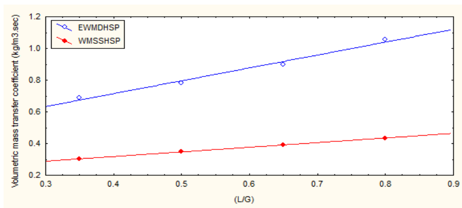
Figure (4): Variation of volumetric mass transfer coefficient with air mass flow rate for the two packs
