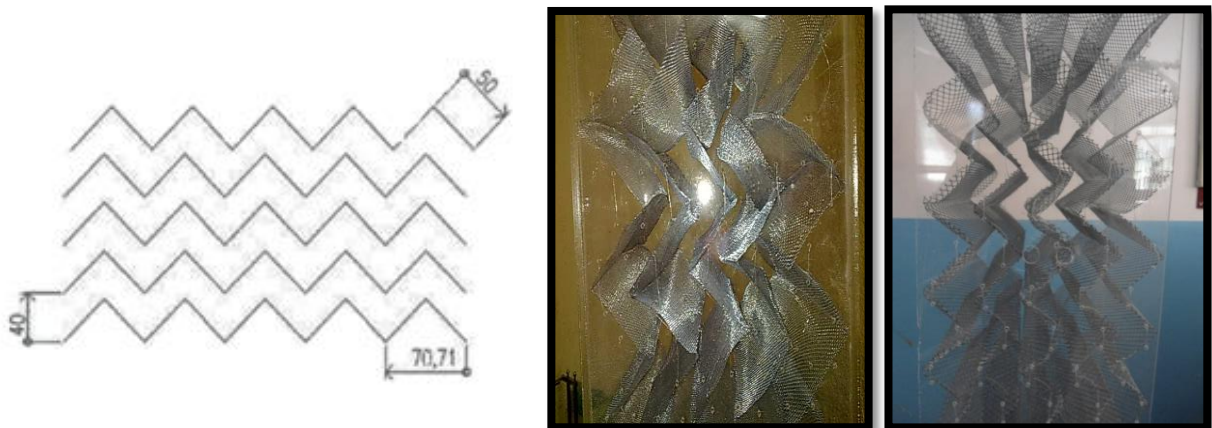
b- Schematic and Photograph is view arrangements of wire mesh of the two packings
