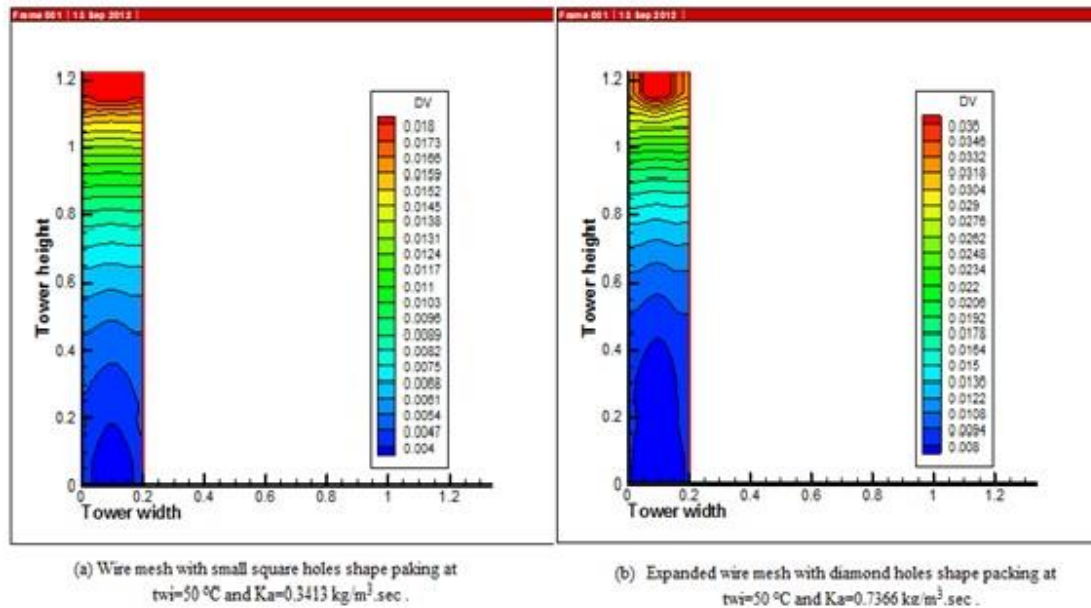
Figure (11) rate of mass transfer distribution of forced draft counter flow water cooling tower.
