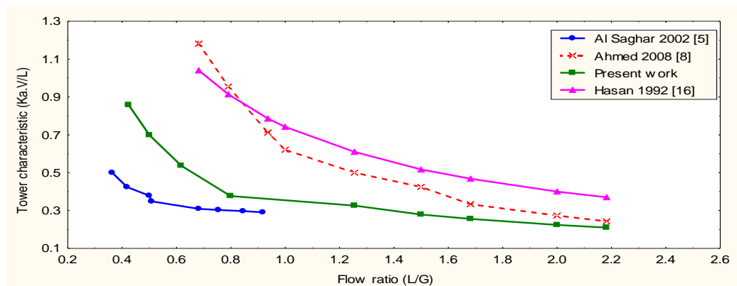
Figure (9): comparison the effect of flow ratio ( L/G ) on the tower characteristic of (EWMDHSP) of the present work with other work.
