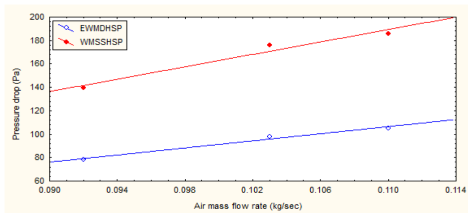
Figure (7): Variation of pressure drop with air mass flow rate for two packs.
