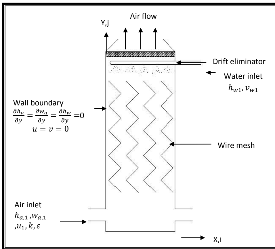
Figure (1) Geometric shape of the water cooling tower
