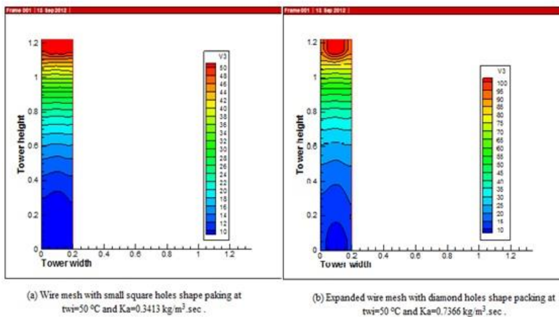
Figure (10) rate of heat transfer distribution of forced draft counter flow water cooling tower.
