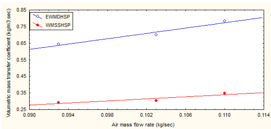
Figure (5): Variation of volumetric mass transfer coefficient with ( L/G ) ratio for two packs.
