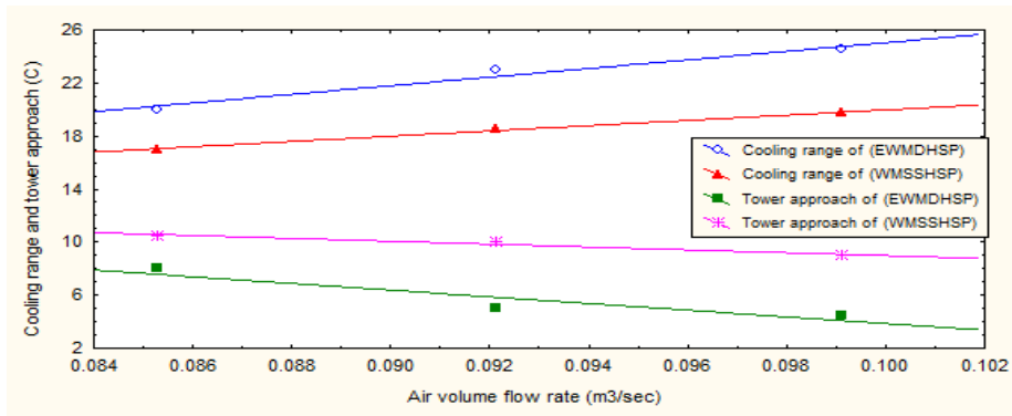
Figure (6): Variation of cooling range and tower approach with air volume flow rate for two packs.
