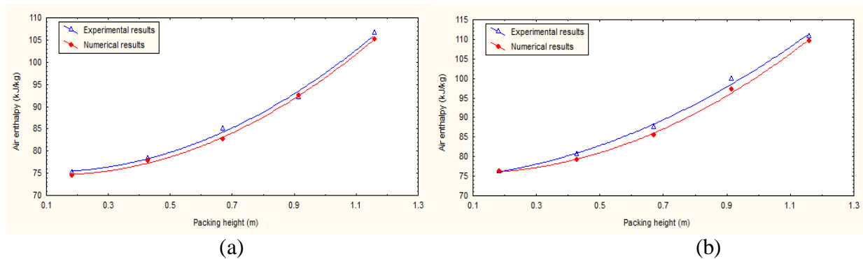
(a) Wire mesh with small square holes shape packing at t_{wi}=53\text{ }^{\circ}\text{C} and Ka=0.2451\text{ kg/m}^3\cdot\text{sec} .
